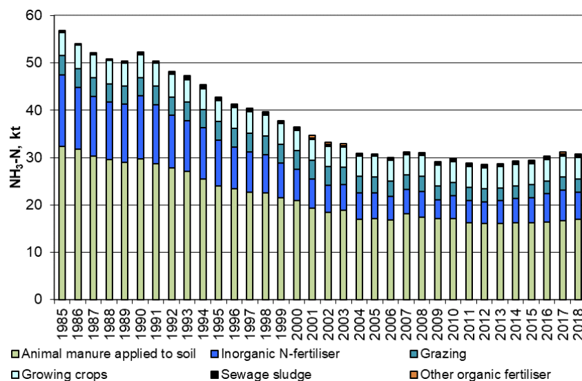
Figure 2.4 \text{NH}_3 -N emission from animal manure applied to soil, inorganic N fertiliser, grazing, growing crops, sewage sludge and other organic, 1985-2018.
