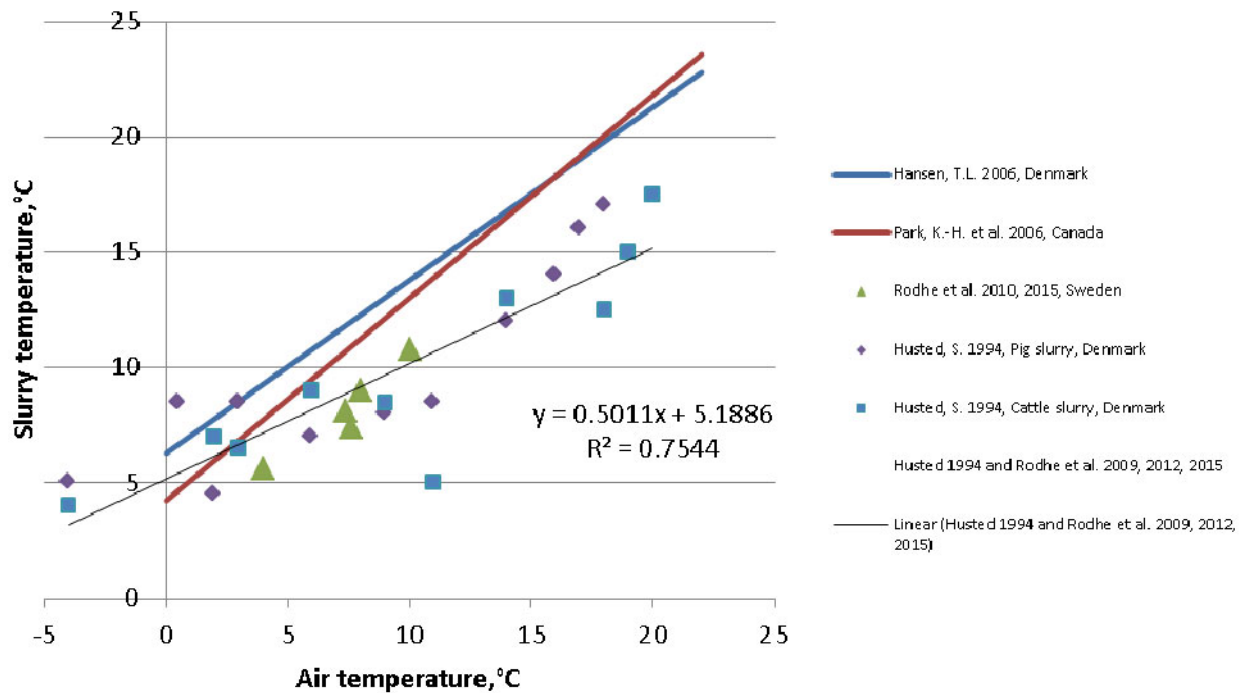
Figure 11.4 Measured and modelled slurry temperatures in outdoor storage tanks.
