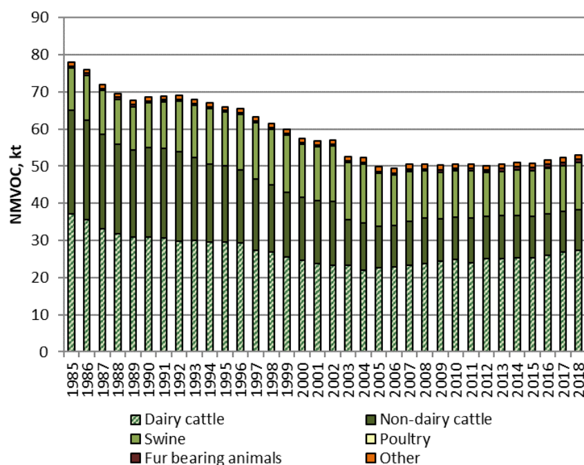
Figure 9.1 Emission of NMVOC from manure management, 1985-2018.
