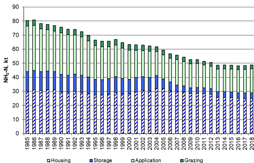
Figure 2.3 NH 3 -N emissions from animal manure, 1985 to 2018.
